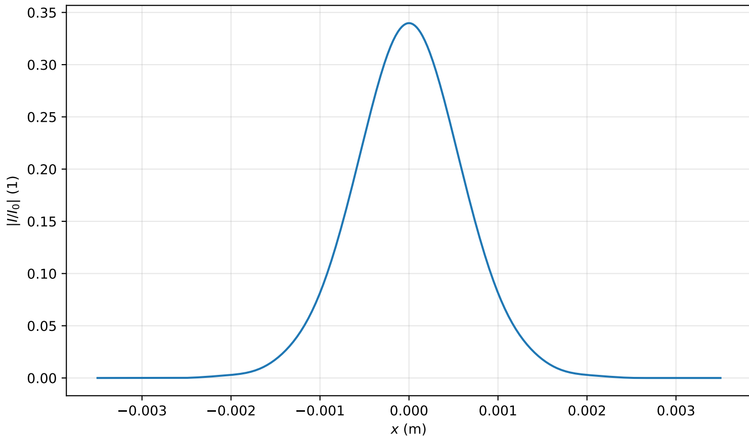
Intensity profile I(x, y = 0, z = 3.901m)/I_0 , P_{in}=0.4P_{cr} , artificial time
